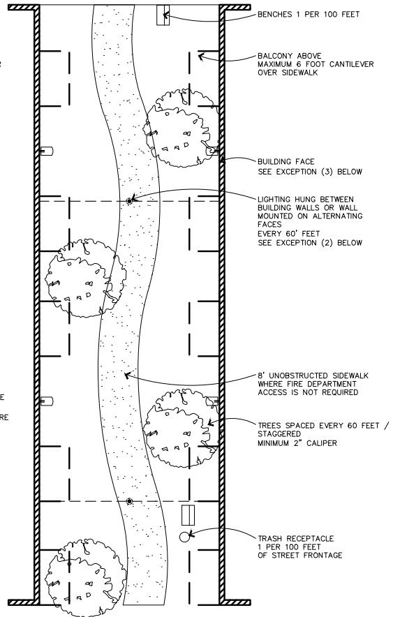
MEWS / PEDESTRIAN WAY WITHOUT FIRE DEPARTMENT ACCESS
